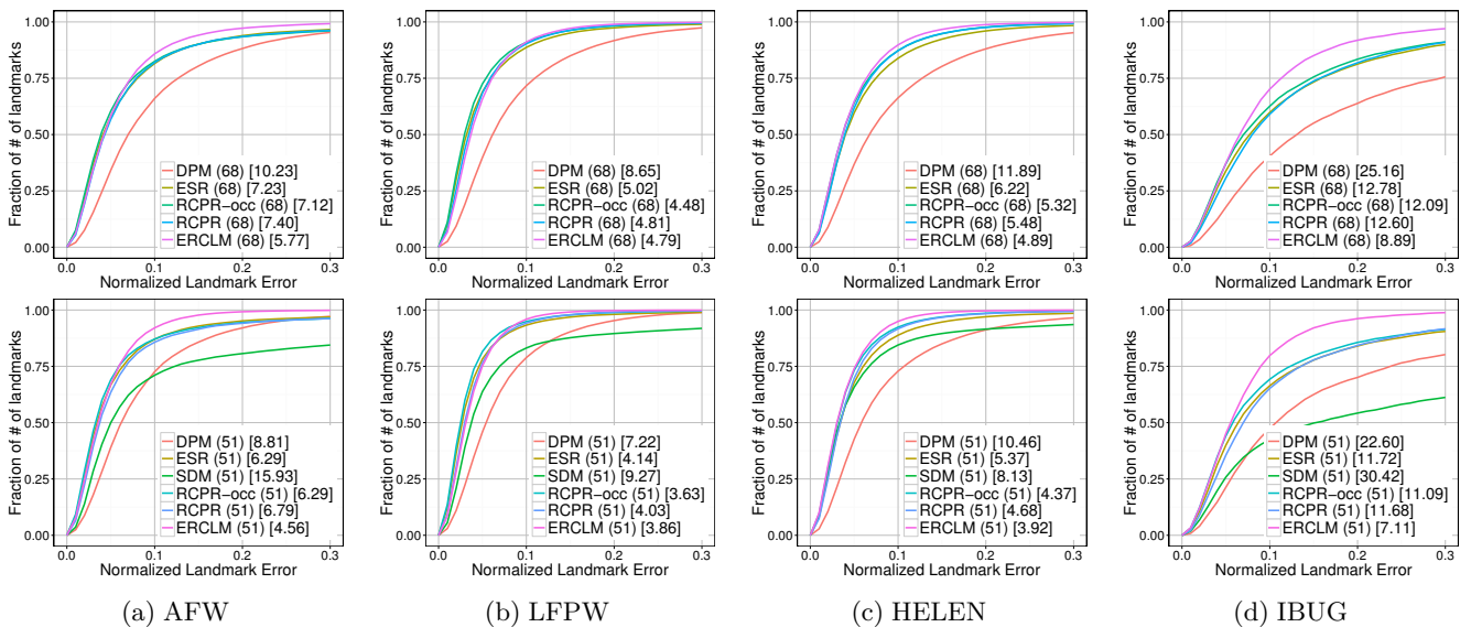
Fig. 1: Cumulative error distribution curves for landmark localization showing the proportion of landmarks that have the Normalized Landmark Error below a given threshold on the AFW , LFPW , HELEN and IBUG datasets. We compare our proposed method to a baseline tree-structured Deformable Parts Model (DPM) [3], Explicit Shape Regression (ESR) [4], Robust Pose Regression (RCPR) [5] and Supervised Descent Method (SDM) [6]. We show face alignment results both including (68) and excluding (51) the points on the jawline. The legend reports the MNLE (in %) at a threshold of 0.1. Our method, ERCLM, shows good alignment performance, especially in the presence of severe occlusions and demonstrates robust generalization across datasets.
