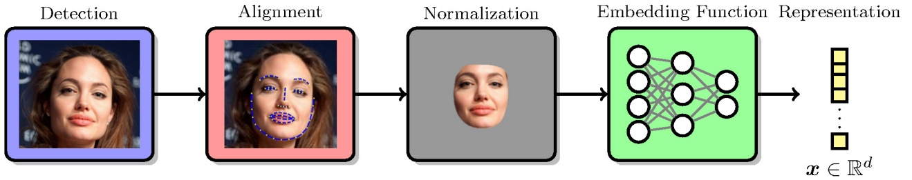
Fig. 1: A typical face representation pipeline comprises of face detection, alignment, normalization and representation or feature extraction. While each of these components affect the capacity of the representation, in this paper, we focus on the capacity of the embedding function that maps a high-dimensional normalized face image to a d -dimensional vector representation.
