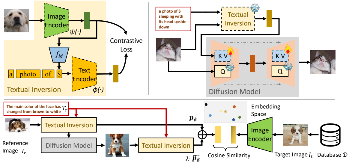
Figure 2. Overview of the proposed Composed Image Generation (CIG). During training, CIG model uses composed prompt embeddings as textual conditions, and learn image information from them. In inference stage, the reference image and delta caption form the composed prompt embedding, which CIG model utilizes to generate pseudo target images. These pseudo target images assist in improving ZS-CIR. Top: the training process, including textual inversion network pretraining (left) and CIG model pertaining (right); bottom: inference process for CIR.
