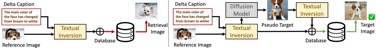
Figure 1. Zero-Shot Composed Image Retrieval vs. Pseudo Target-Aided Composed Image Retrieval. Conventional ZS-CIR methods map the image latent embedding into the token embedding space by textual inversion. The proposed Pseudo Target-Aided method provide additional information for composed embeddings from pseudo-target images.
